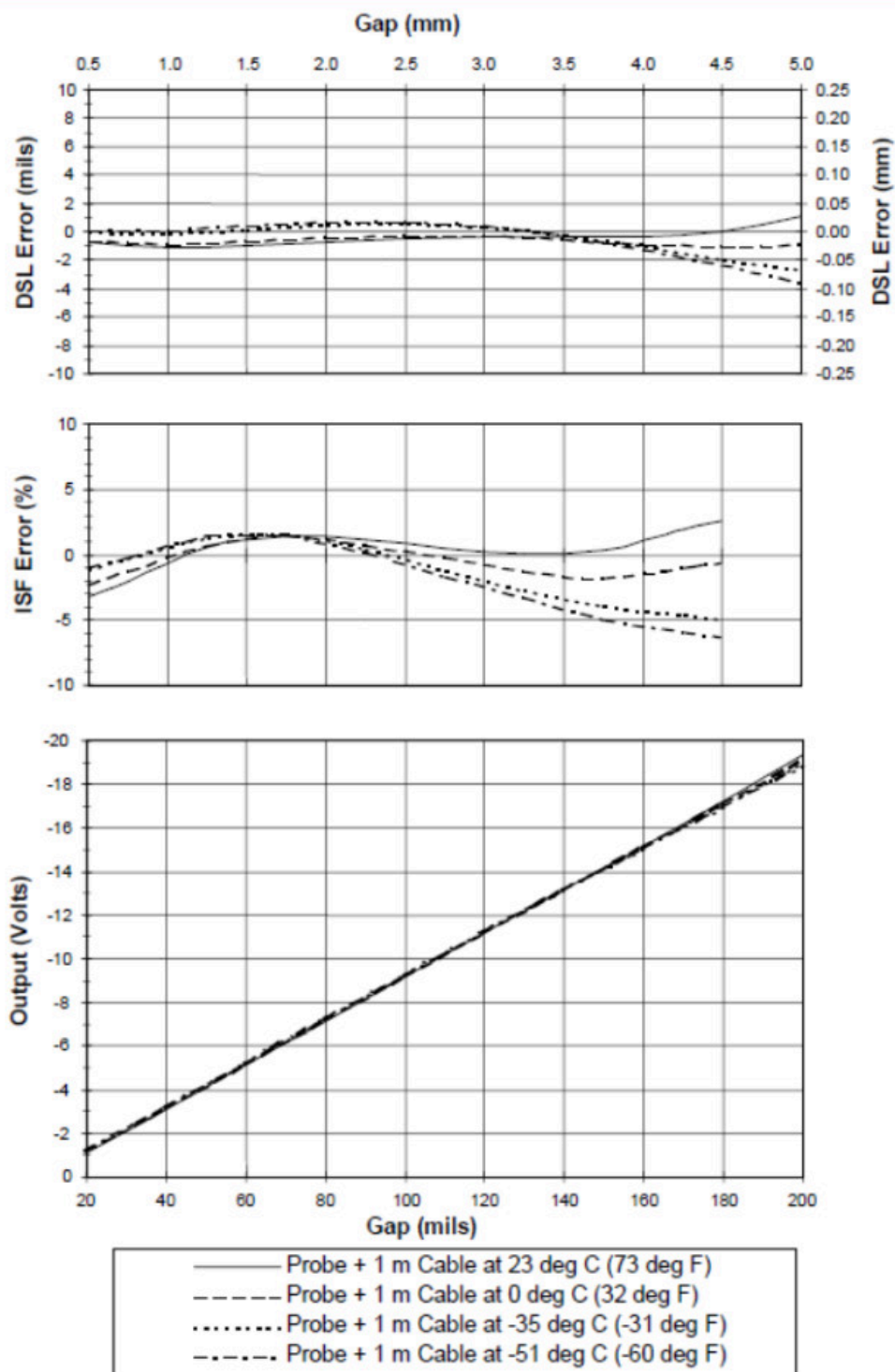
Figure 3: Typical 3300 XL 11 mm Probe + 1m Cable @ Low Temperature (Proximitior Sensor + 4m of Extension Cable @ 25 °C)
