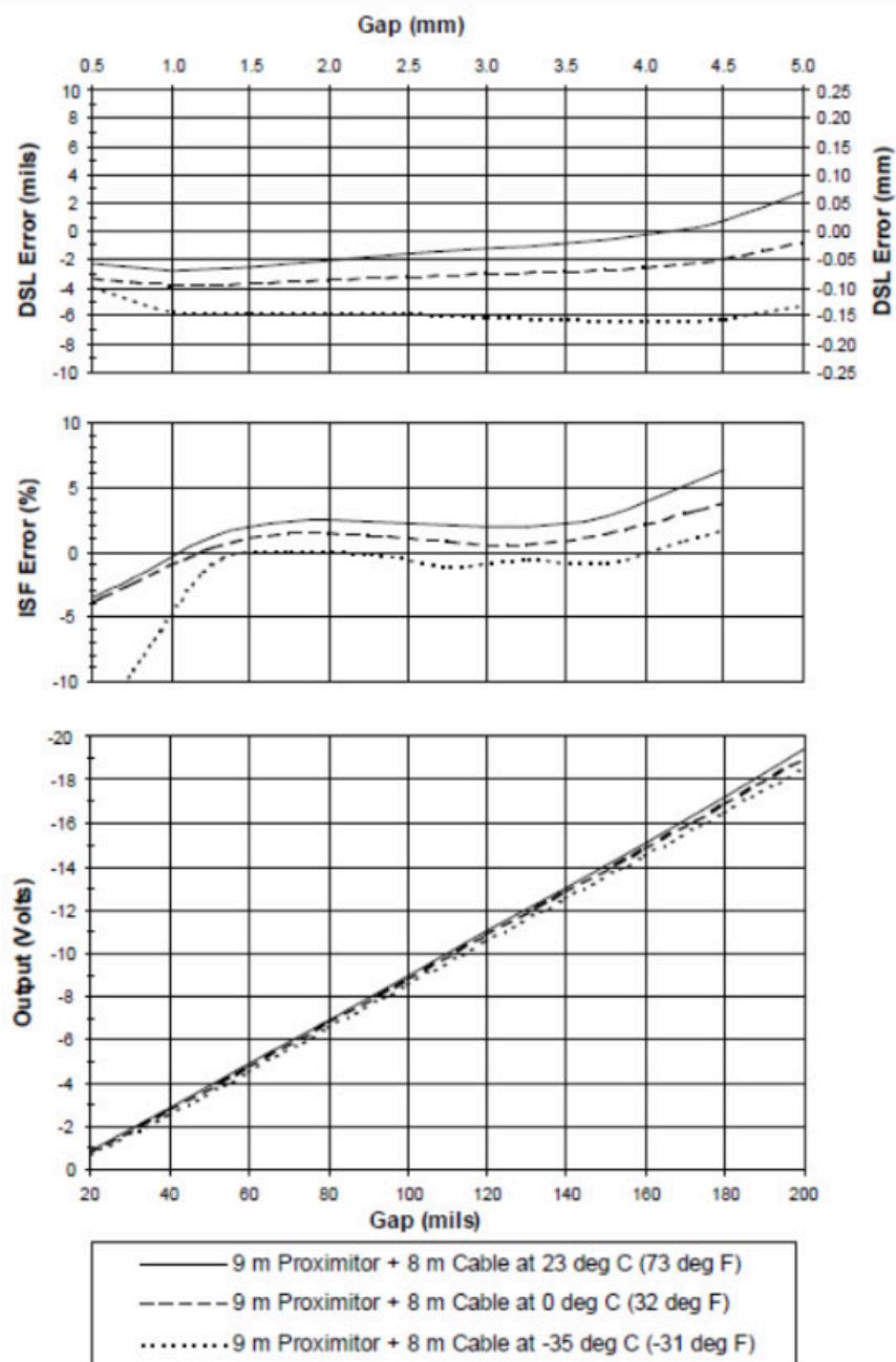
Figure 7: Typical 3300 XL 11 mm 9 m Proximitior Sensor with 8 m of Extension Cable @ Low Temperature
